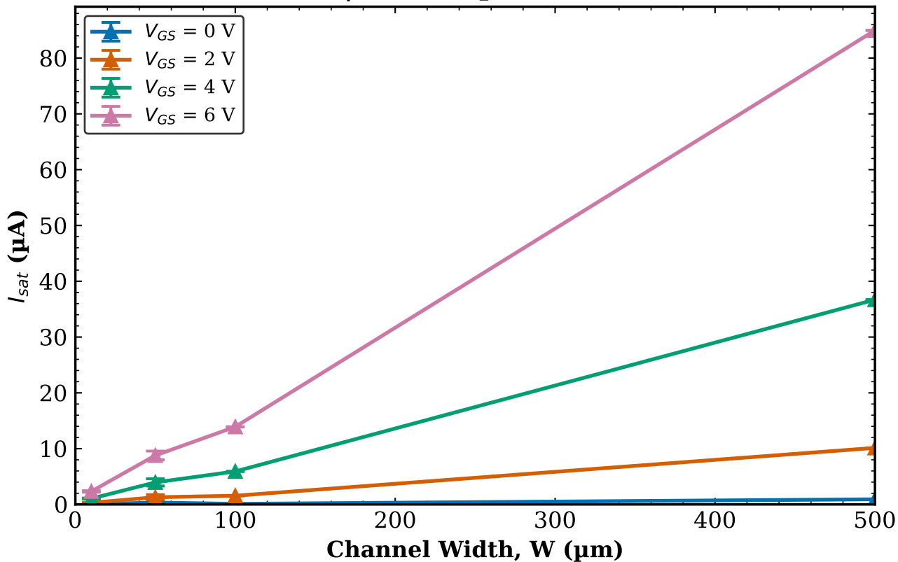
TFT1 Combined (Tr. 1 & 2) I_{sat} vs W | L = 80\text{ }\mu\text{m} (mean \pm std)
